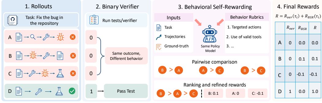
Figure 1: Overview of Behavioral Self-Rewarding (BSR). Binary rewards provide no contrast when trajectories share the same verifier outcome, while BSR ranks them within the outcome group to recover a bounded learning signal.
