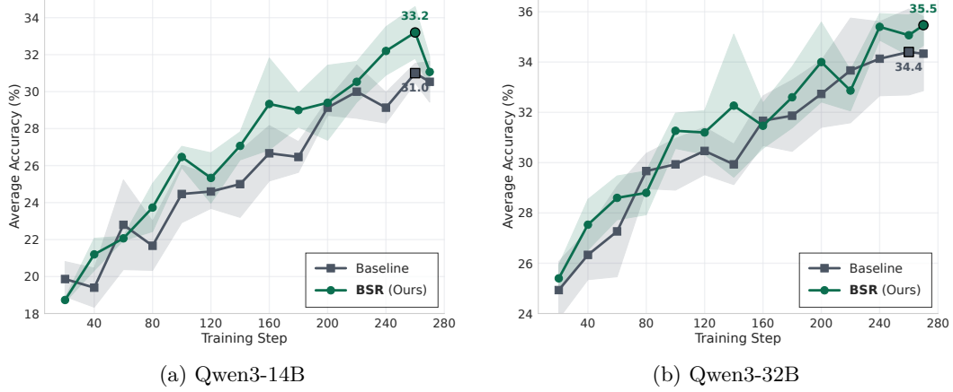
Figure 2: SWE-bench Verified evaluation accuracy over training for Qwen3-14B and Qwen3-32B. Each point averages three evaluation runs.
