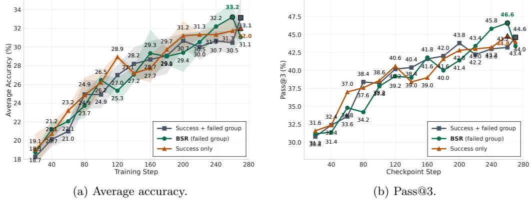
Figure 6: Verifier-outcome-bucket ablation on SWE-bench Verified while training Qwen3-14B. We compare applying BSR to failed trajectories only, successful trajectories only, and both successful and failed trajectories.
