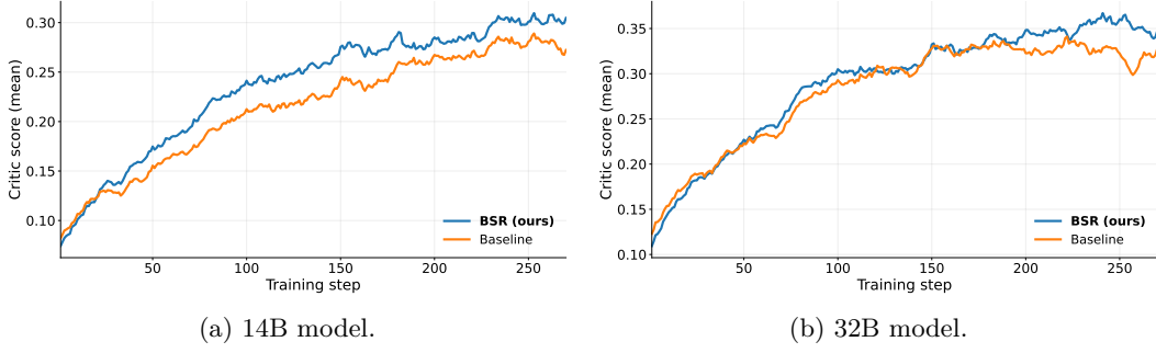
Figure 3: Mean critic scores on training set for BSR and the baseline. Curves are smoothed with EMA with a span of 31 (Note here the critic score is just the score from the execution verifier).
