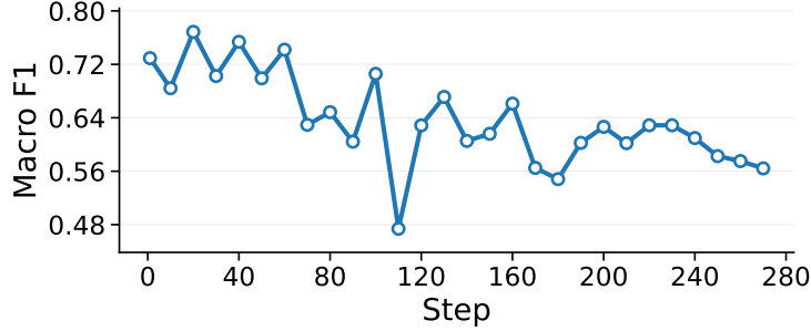
Figure 8: Agreement with Kimi-2.5 on sampled pairwise trajectory comparisons over training, measured by macro F1. At each evaluation point, 200 on-policy comparison pairs are sampled and re-evaluated using Kimi-2.5 as an external reference judge.
