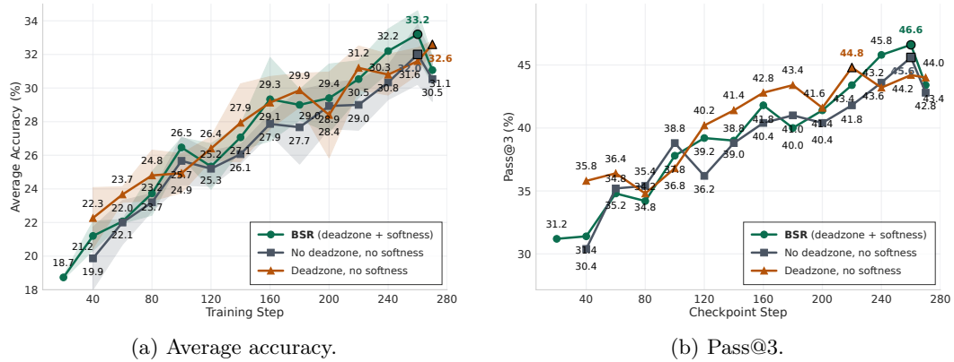
Figure 7: Reward-mapping ablation on SWE-Bench Verified while training Qwen3-14B. We compare the full BSR reward mapping against variants without the deadzone and/or softness.
